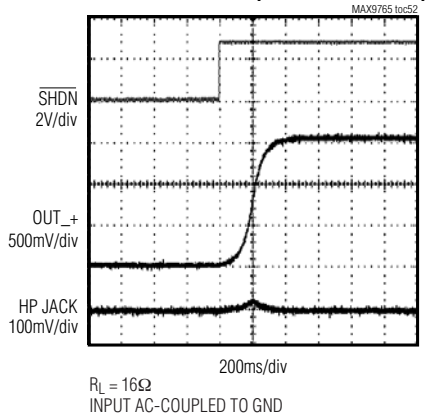
EXITING SHUTDOWN (HEADPHONE MODE)
