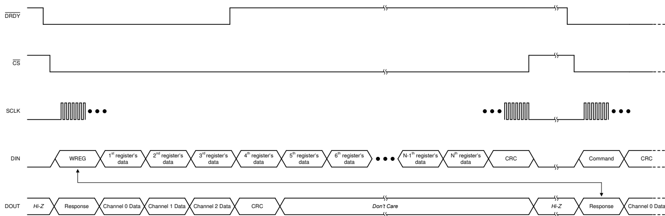
Figure 8-25. Writing Registers
