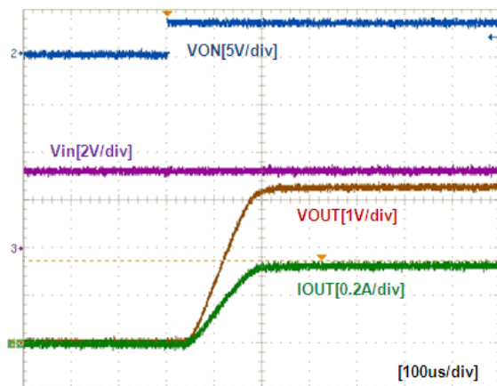
Figure 17. Turn-On Response – FPF1203 / 04 (V IN =3.3 V, C IN =1 μF, C OUT =0.1 μF, R L =10 Ω)
