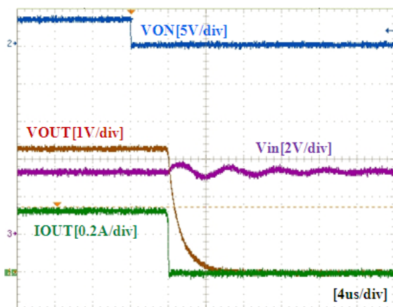
Figure 18. Turn-Off Response – FPF1203 (V IN =3.3 V, C IN =1 μF, C OUT =0.1 μF, R L =10 Ω)
