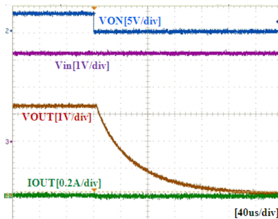
Figure 19. Turn-Off Response – FPF1203 (V IN =3.3 V, C IN =1 μF, C OUT =0.1 μF, R L =500 Ω)
