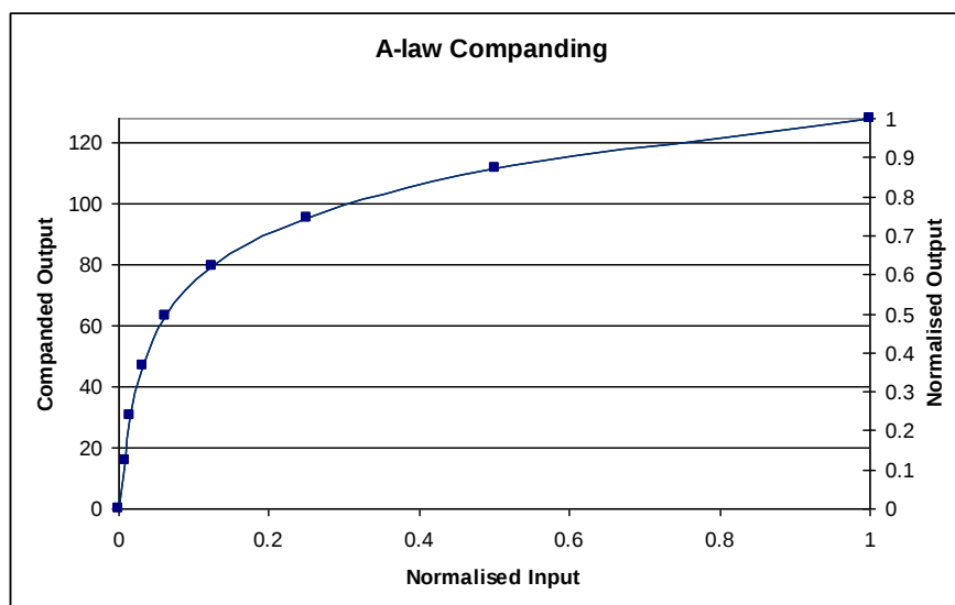
Figure 58 A-Law Companding
