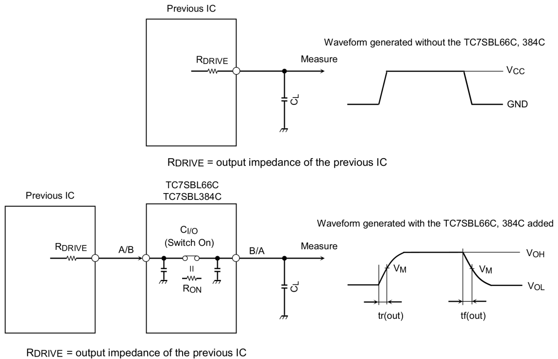
Fig. 12.1 Calculation Circuit
