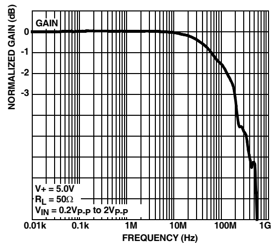
FIGURE 14. FREQUENCY RESPONSE
