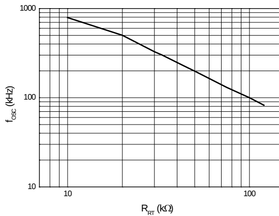
f_{osc} vs. R_{RT}
