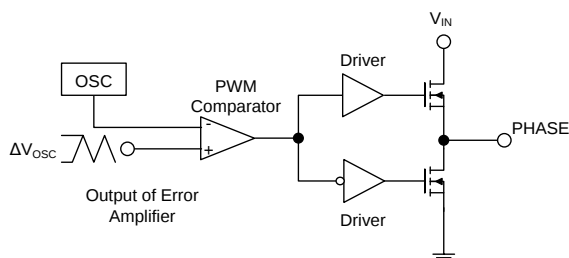
Figure 8. The PWM Modulator
