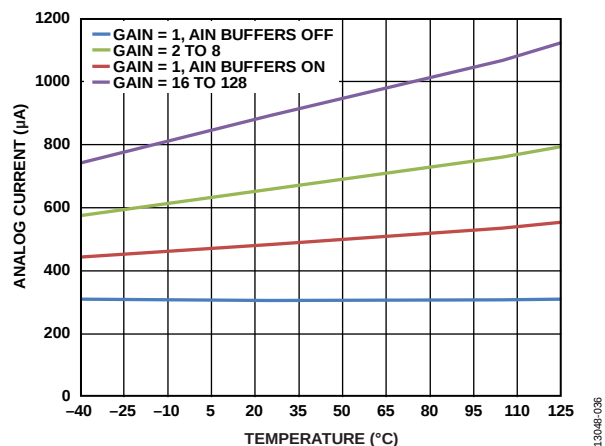
Figure 36. Analog Current vs. Temperature (Full Power Mode)
