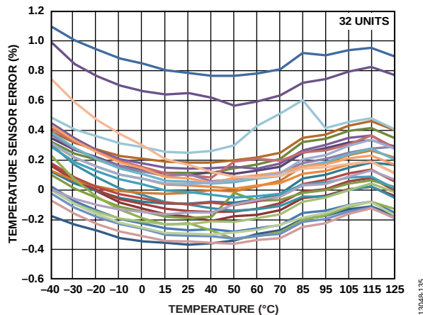
Figure 128. Temperature Sensor Error vs. Temperature
