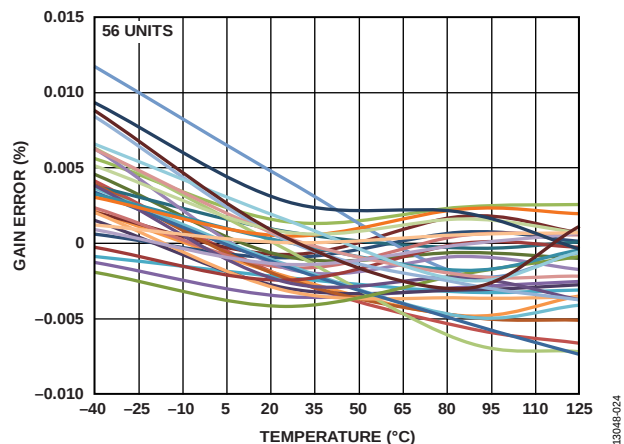
Figure 24. Input Referred Gain Error vs. Temperature (Gain = 8)
