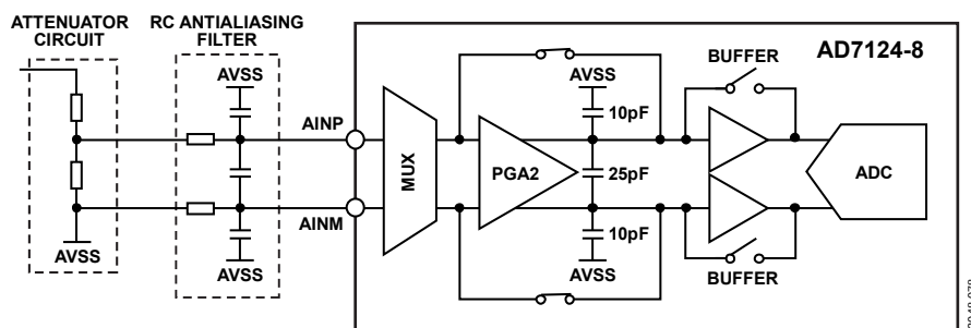
Figure 76. Input Schematic
