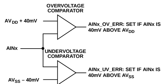
Figure 122. Analog Input Overvoltage/Undervoltage Monitors
