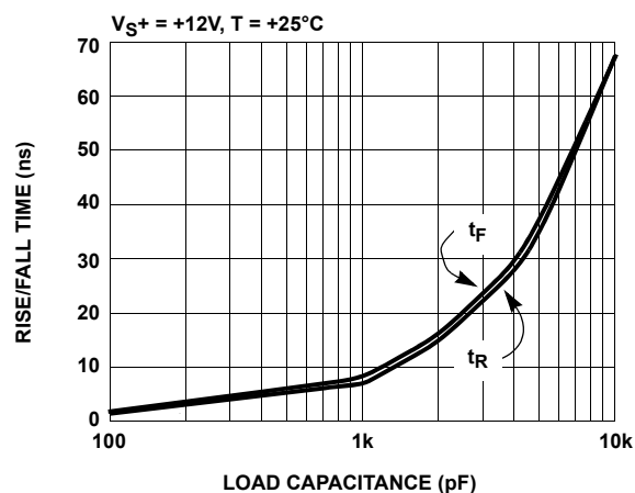
FIGURE 8. RISE/FALL TIME vs LOAD CAPACITANCE
