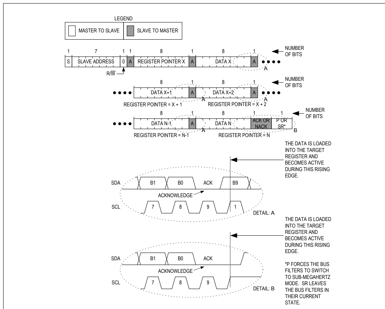
Figure 24. Writing to Sequential Registers X to N
