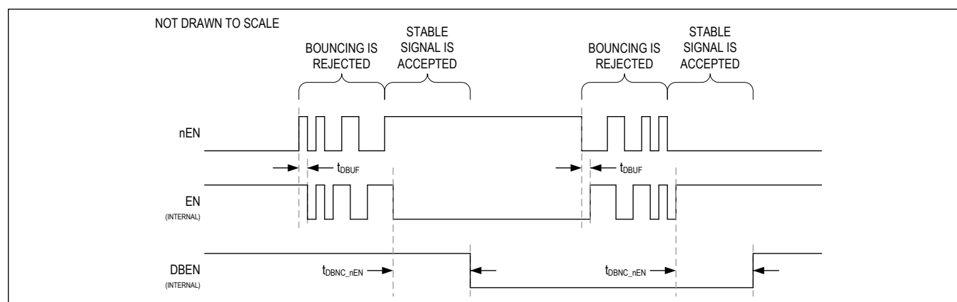
Figure 12. Debounced Inputs
