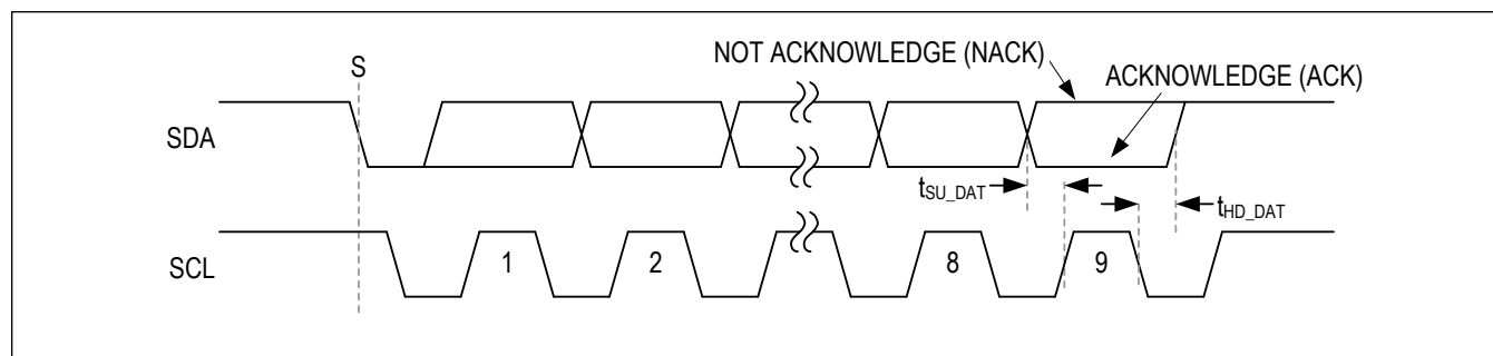
Figure 21. Acknowledge Bit
