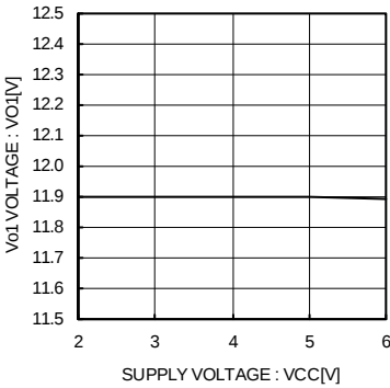
Fig. 15 Vo1 Line Regulation
