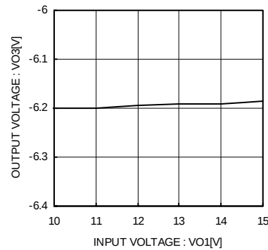
Fig. 22 Negative-side Charge Pump Line Regulation
