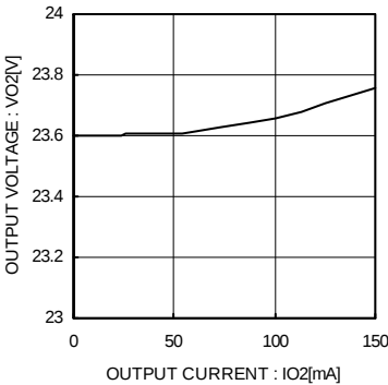
Fig. 21 Vo2 Load Regulation
