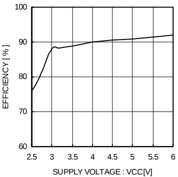
Fig. 18 Efficiency vs Power Supply Voltage
