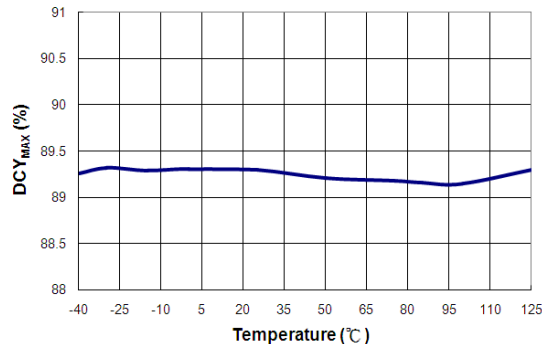
Figure 16. Maximum Duty Cycle ( DCY_{MAX} ) vs. Temperature
