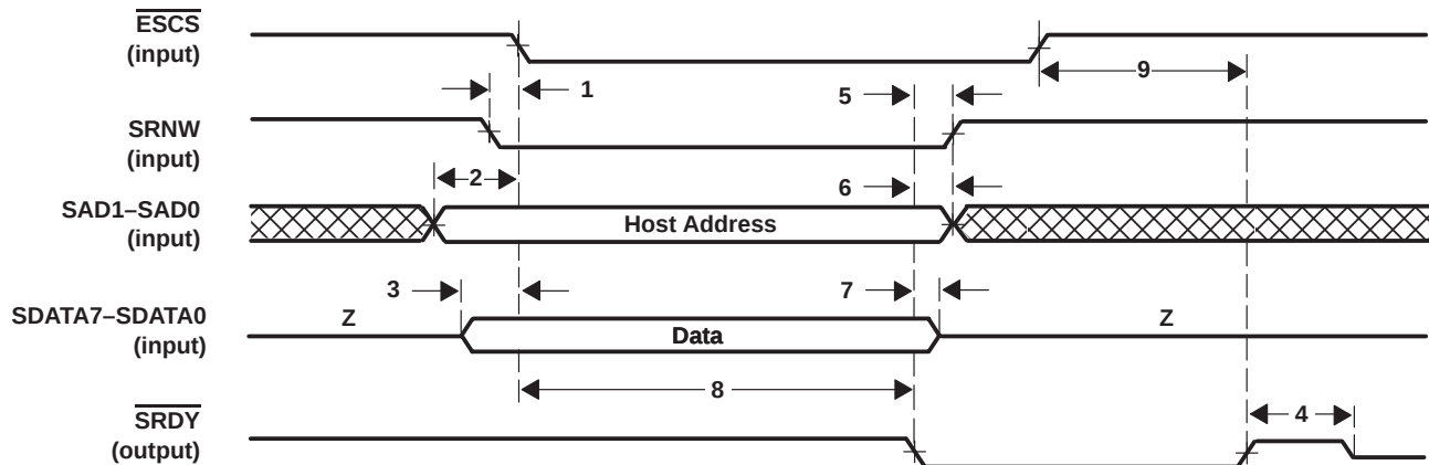
Figure 23. DIO Write Cycle
