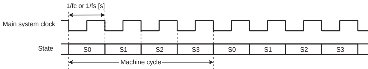
Figure 2-5 Machine Cycle
