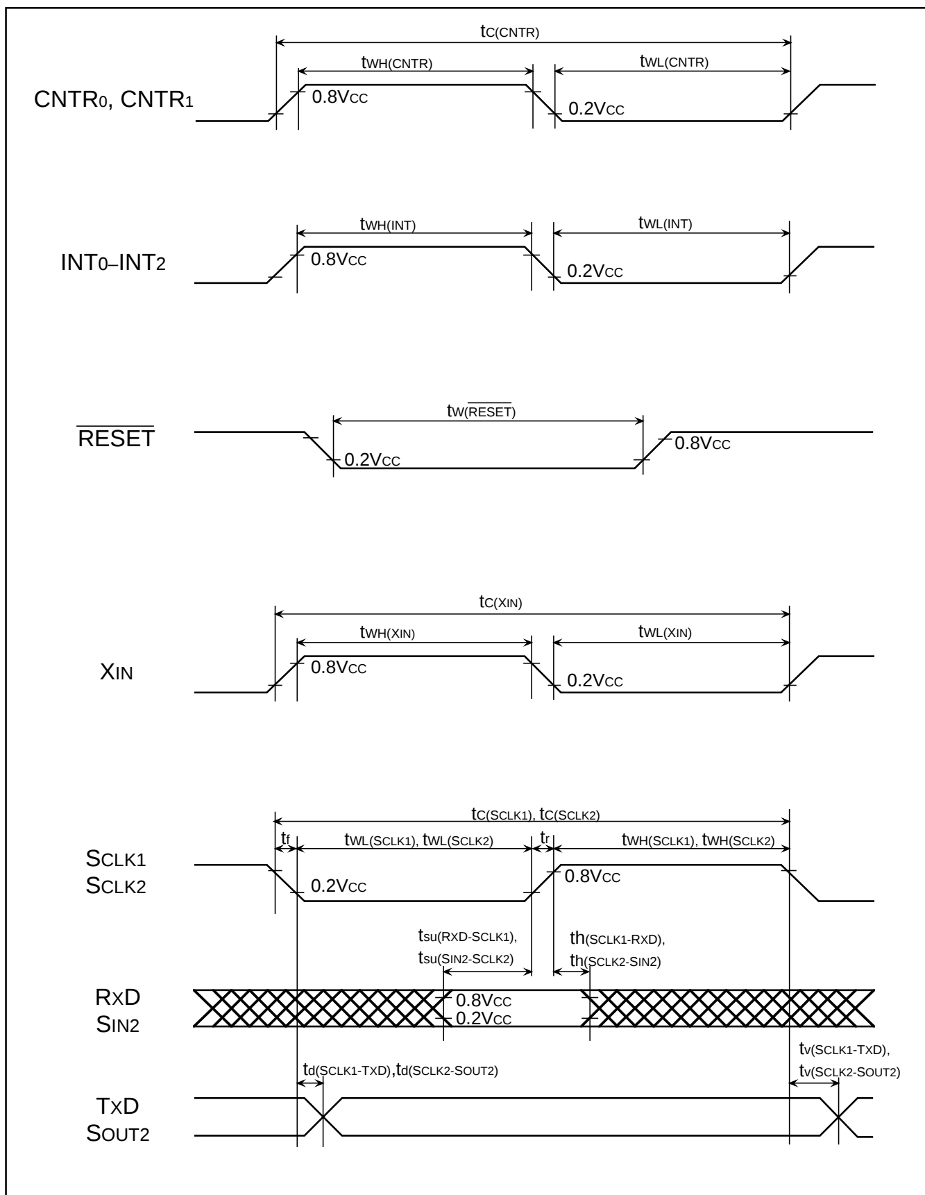
Fig. 70 Timing diagram
