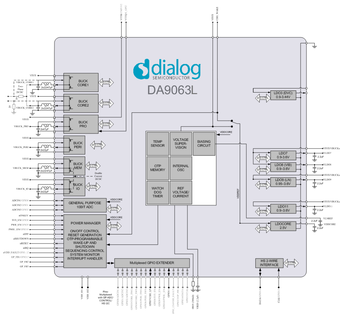
Figure 1: Block Diagram
