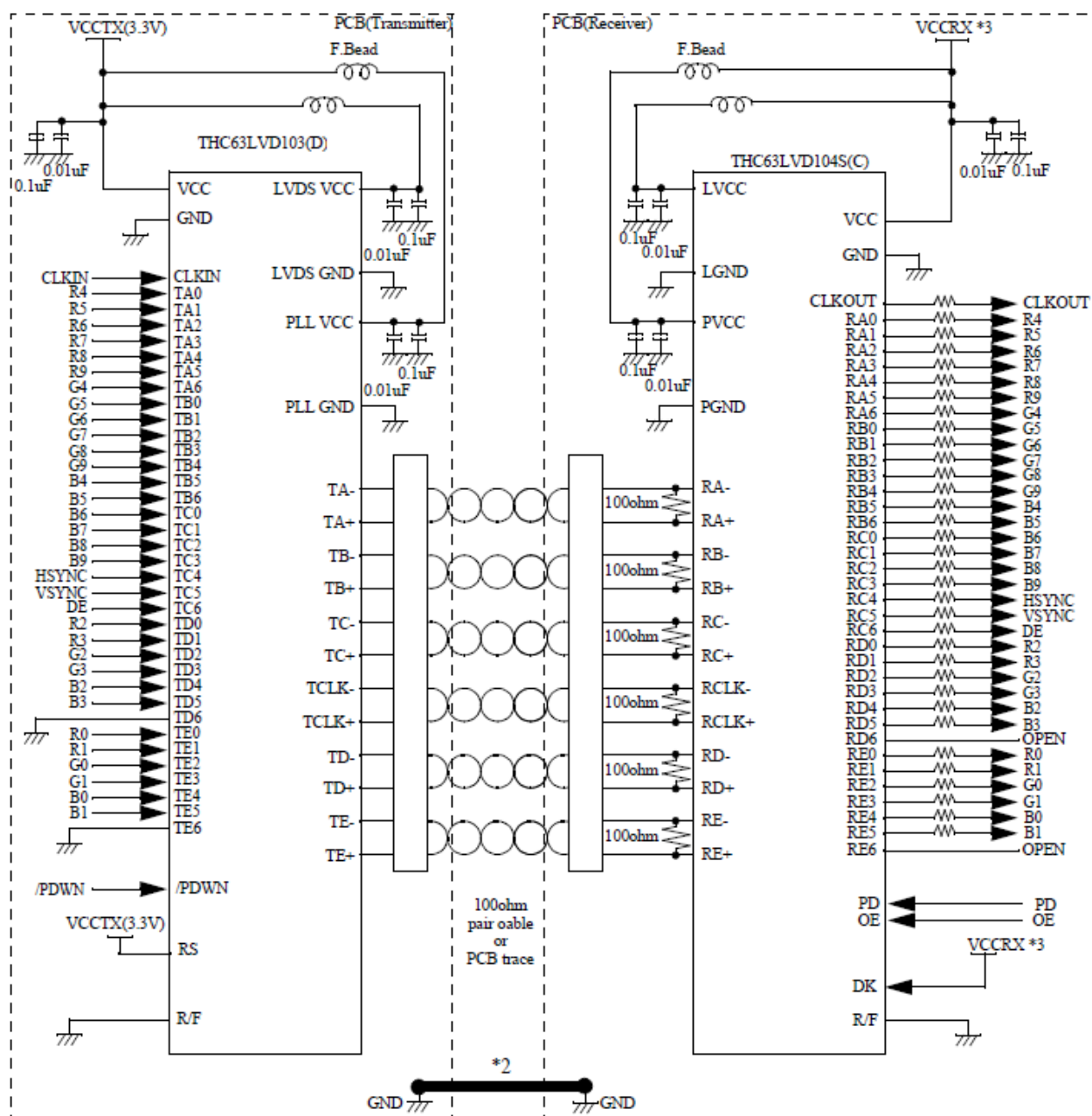
Figure 13. Typical Connection Diagram
