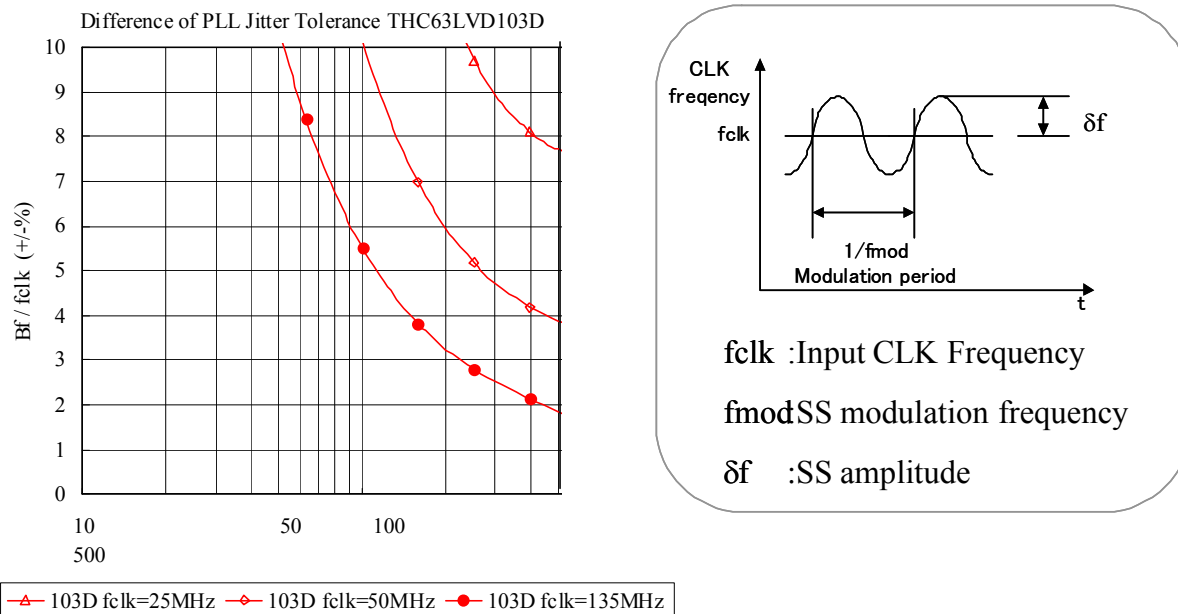
Figure 11. Spread Spectrum Clocking Tolerant
