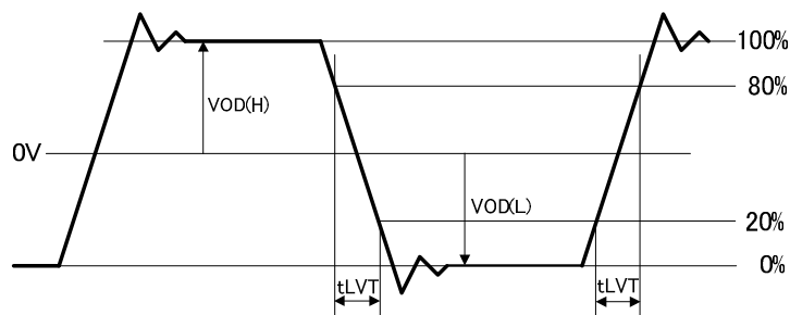
Figure 6. LVDS Output Load and Transition Time
