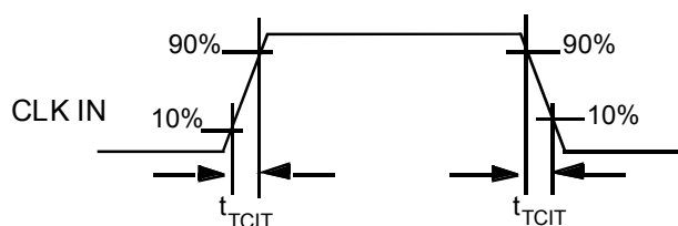
Figure 5. CLKIN Transmission Time
