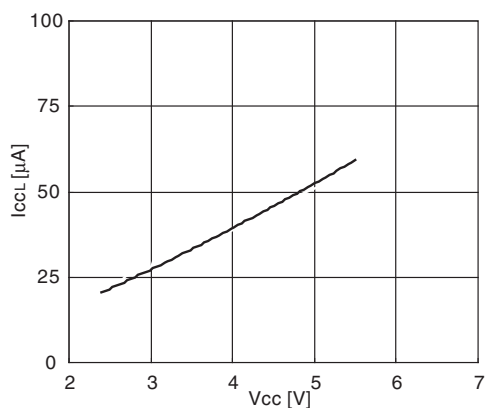
I CCL - V CC T_A = +25^\circ\text{C} F_{MPL} = 16 kHz (divided by 2) Subclock mode with the external clock operating
