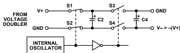
Figure 14. Charge Pump Voltage Inverter
