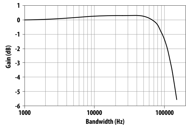
Figure 14 Frequency Response
