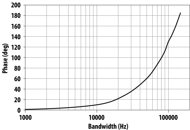
Figure 15 Phase Response
