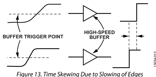
Figure 13. Time Skewing Due to Slowing of Edges
