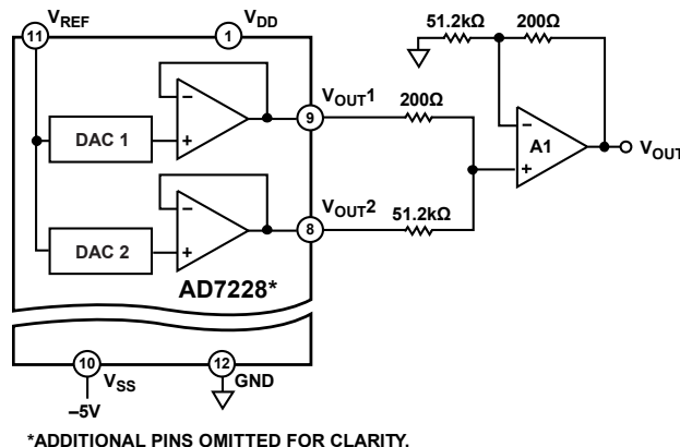
Figure 15. Coarse/Fine Adjust Circuit
