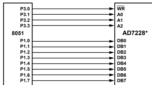
Figure 22. AD7228 to 8051 Interface
