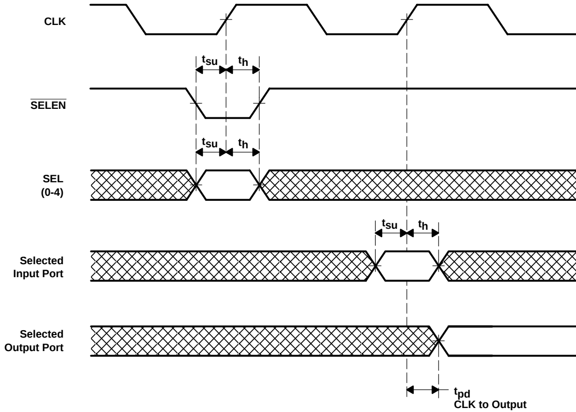
timing diagram
