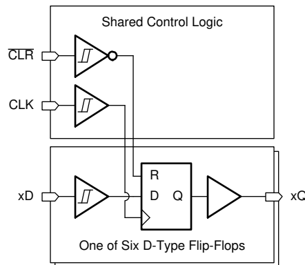
Figure 8-1. Logic Diagram (Positive Logic) for SN74HCS174-Q1
