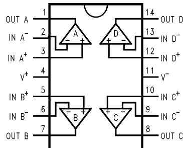
14-Pin TSSOP
