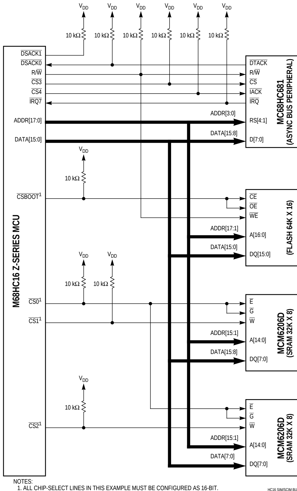
Figure 5-10 MCU Basic System
