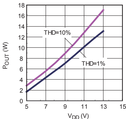
V_{DD} vs. P_{OUT}
