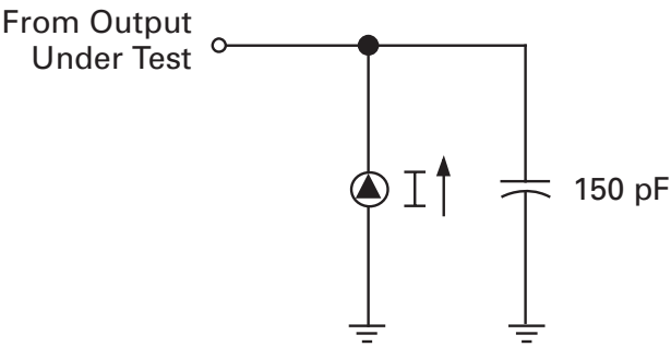
Figure 7. Test Load Diagram
