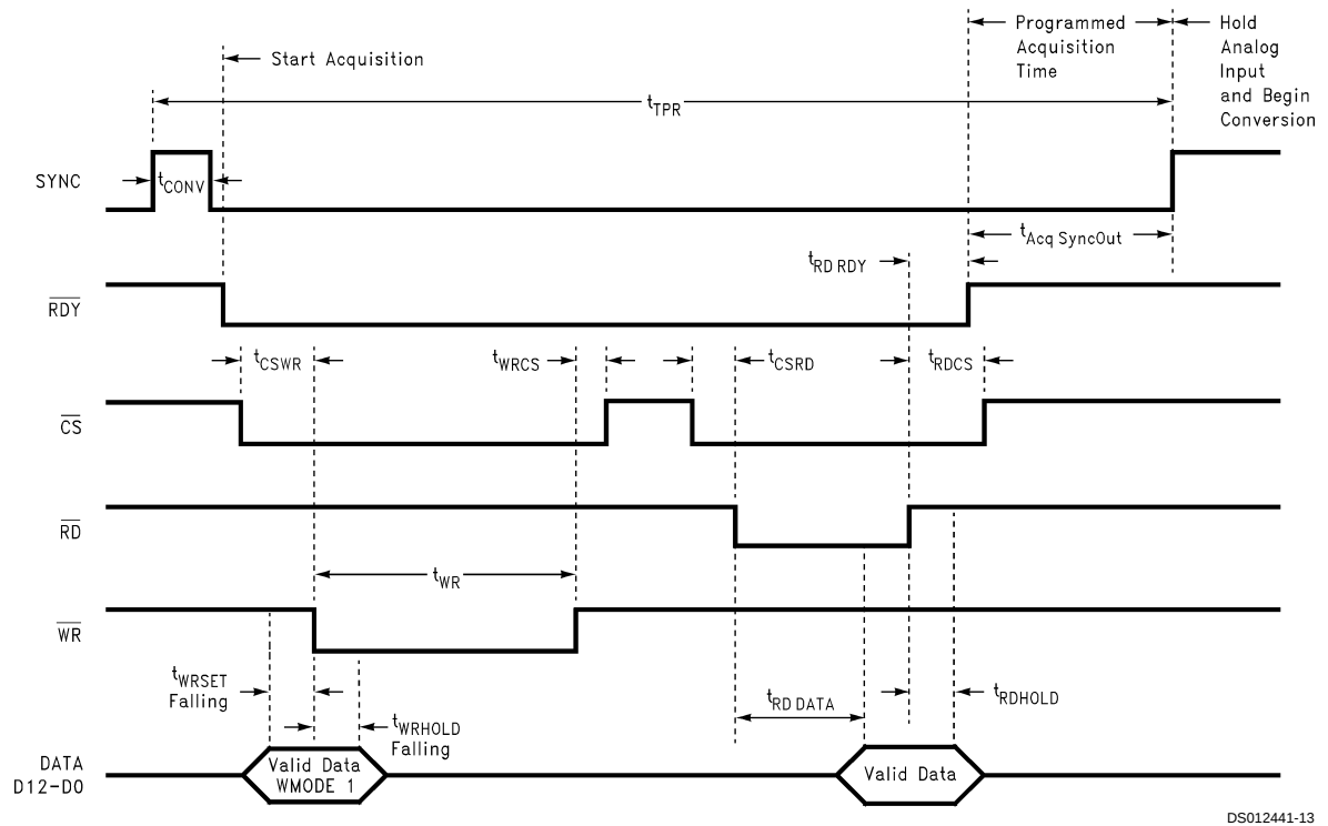
FIGURE 9. Sync-Out Write (WMODE = 1, BW = 1), Read and Convert Cycles
