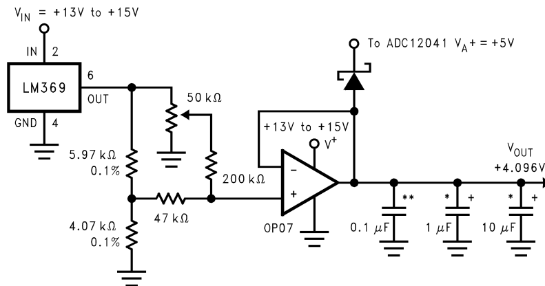
FIGURE 20. Low Drift Extremely Stable Reference Circuit
