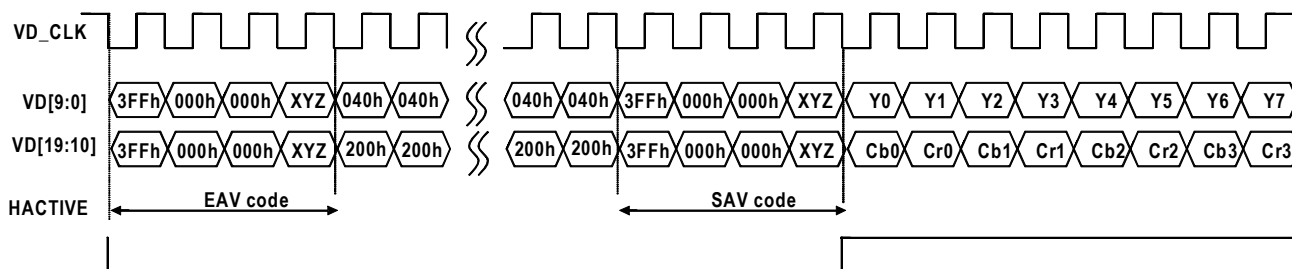
FIGURE 7. BT.1120 FORMAT
