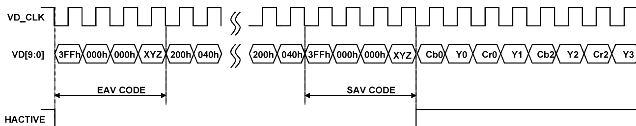
FIGURE 4. BT.656 FORMAT
