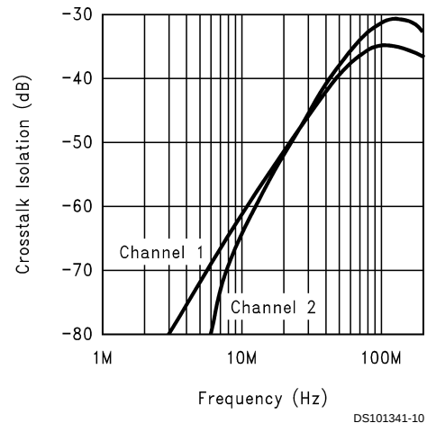
Channel-to-Channel Crosstalk
