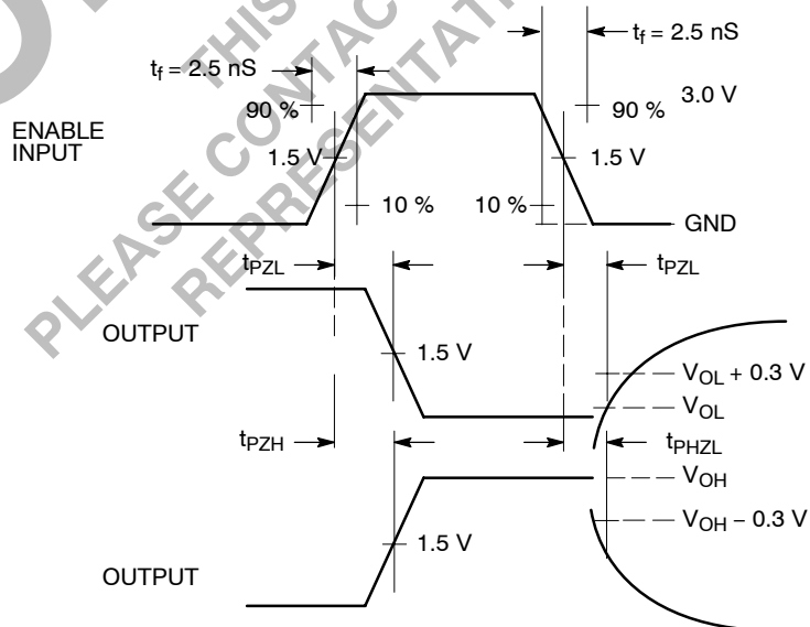
Figure 6. Enable/Disable Delays
