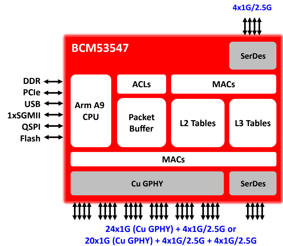
Figure. BCM53547 Block Diagram
