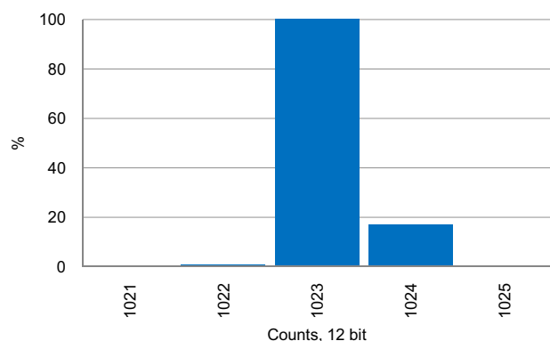
Figure 11-28. SAR ADC Noise Histogram, 100 kps, Internal Reference No Bypass
