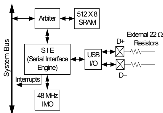
Figure 7-14. USB
