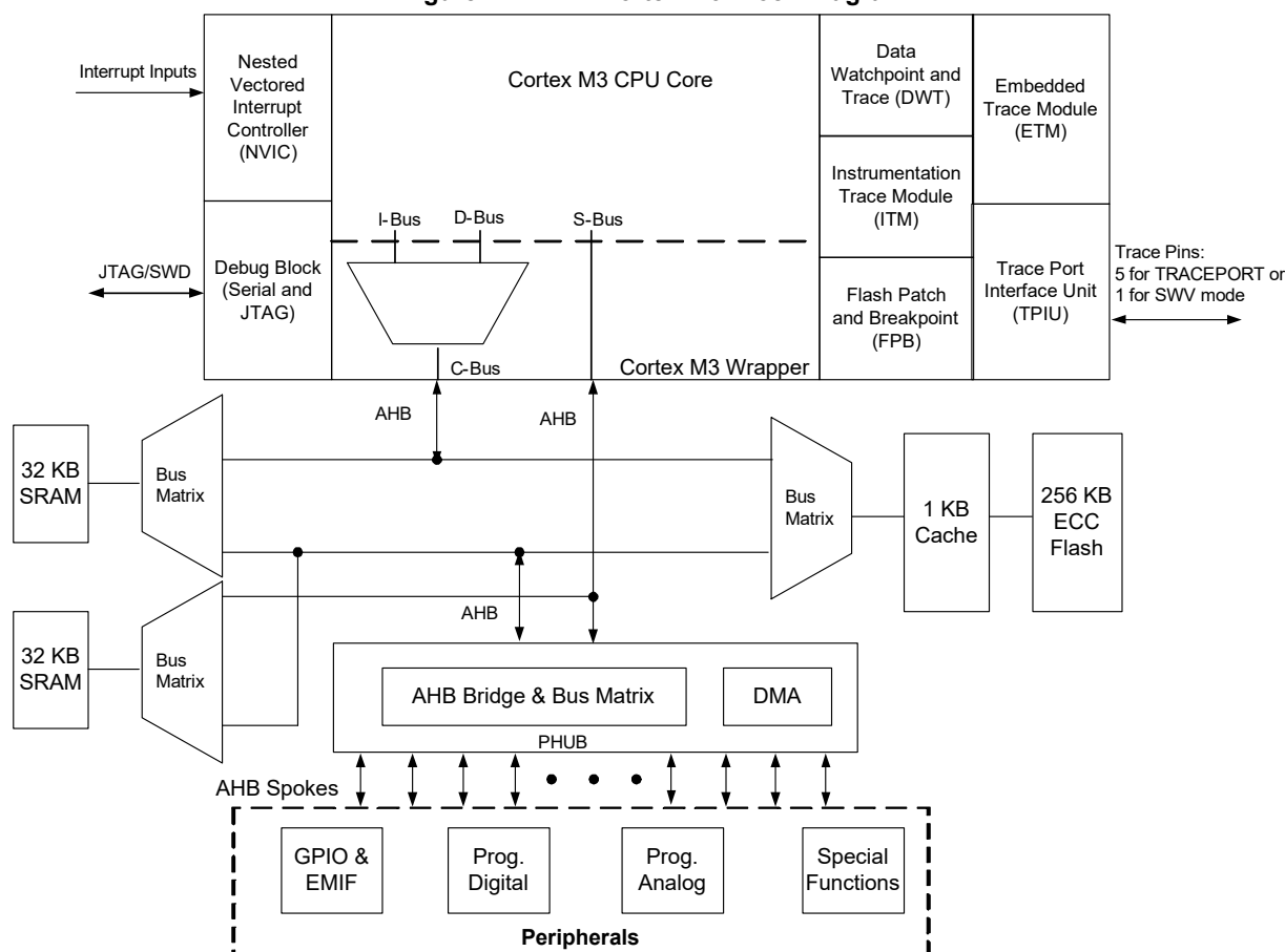
Figure 4-1. ARM Cortex-M3 Block Diagram
