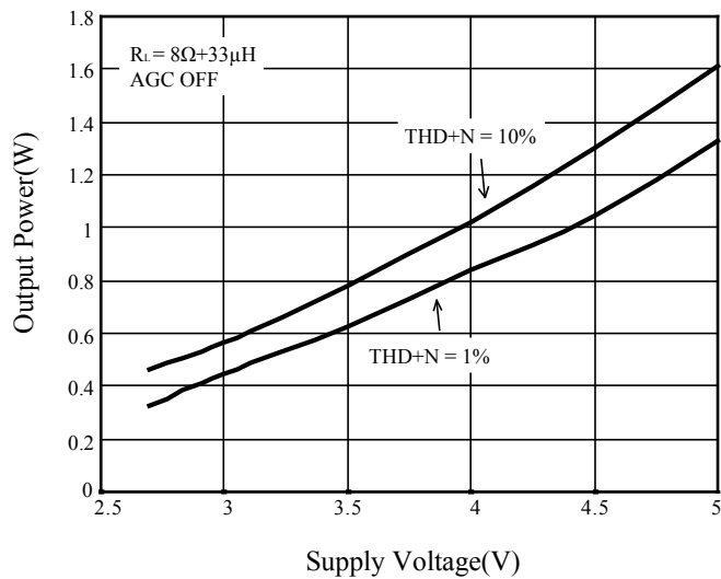
Figure 9 Output Power vs. Supply Voltage
