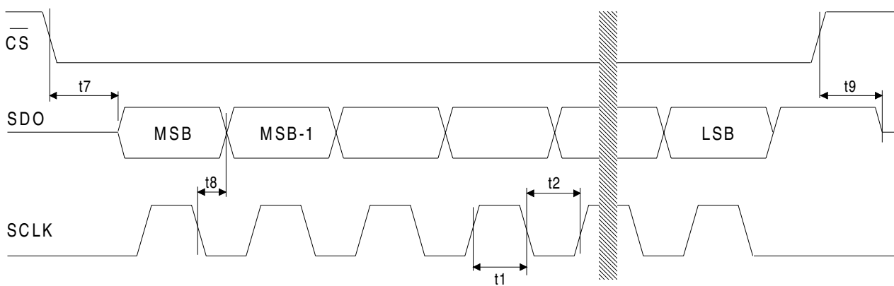
SDO Read Timing (Not to Scale)
