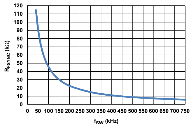
Figure 129. R_{FSYNC} vs Switching Frequency
