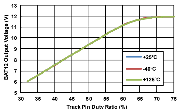
Figure 25. BAT12 Output Voltage (Digital Tracking Mode, FTRK = 150kHz, Buck Mode, DE Mode, Phase Drop Disabled, f_{CLK} = 100kHz)
