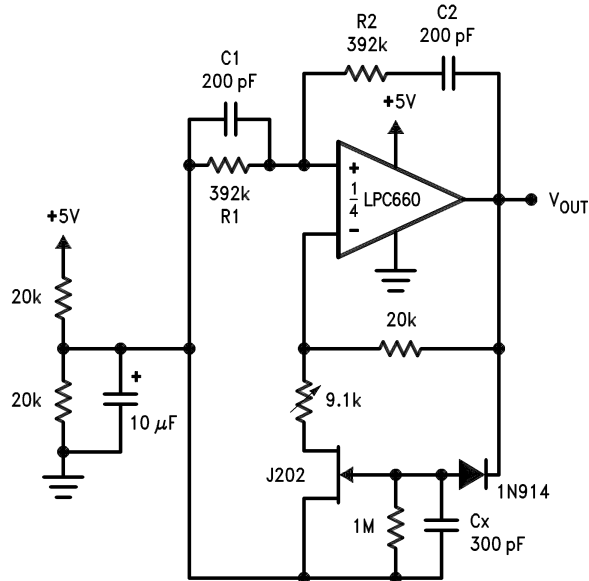
Sine-Wave Oscillator
