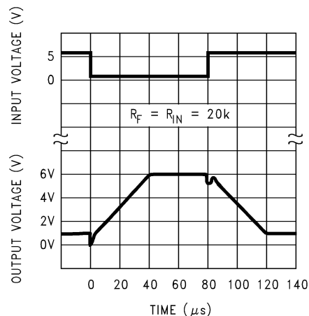
Inverting Large-Signal Pulse Response
