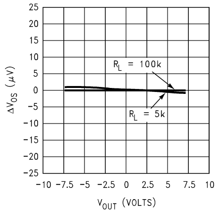
Gain Error ( V_{OS} vs. V_{OUT} )
