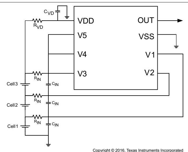
Figure 9-10. 3-Series Cell Configuration with Fixed Delay
