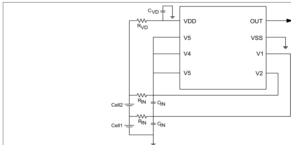
Figure 9-11. 2-Series Cell Configuration with Internal Fixed Delay
