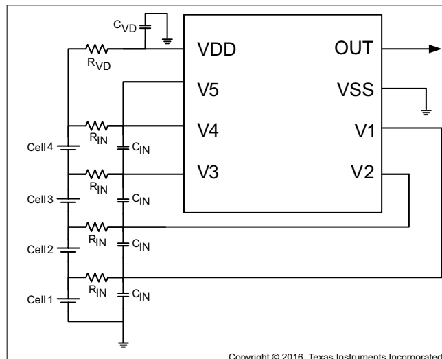
Figure 9-9. 4-Series Cell Configuration
