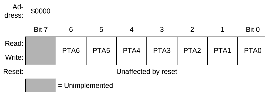
Figure 14-2. Port A Data Register (PTA)
