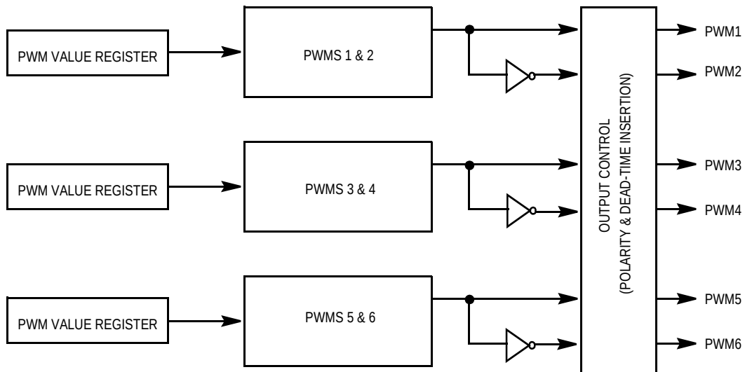
Figure 9-11. Complementary Pairing
