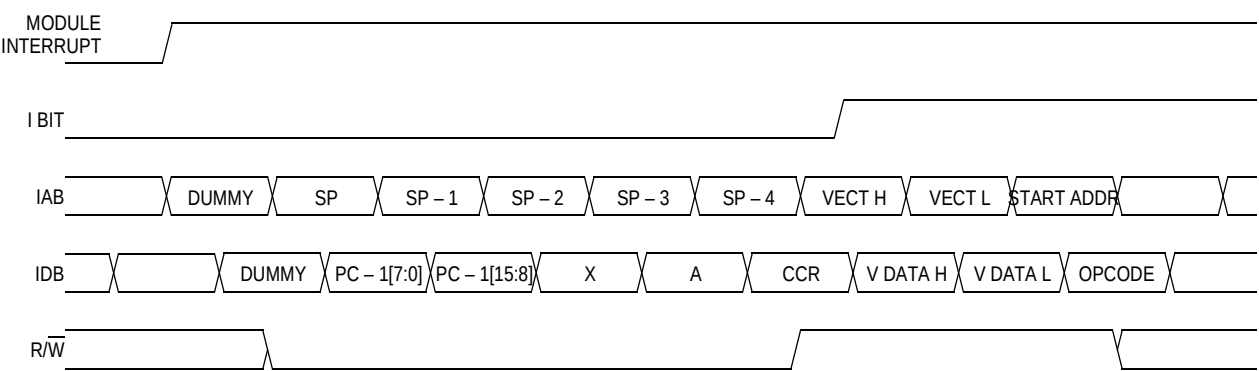
Figure 7-8. Interrupt Entry
