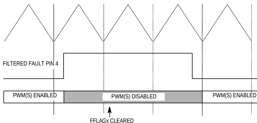
Figure 9-26. PWM Disabling in Manual Mode (Example 2)
