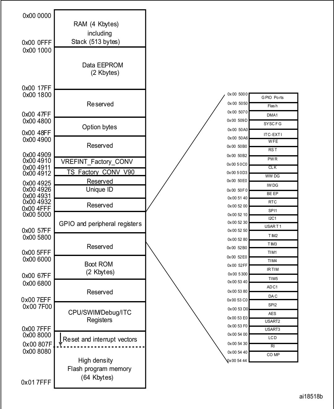
Figure 5. Memory map
