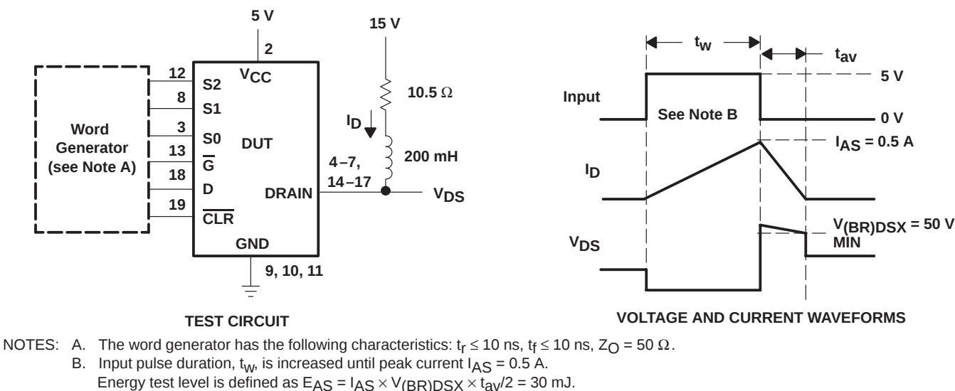
Figure 4. Single-Pulse Avalanche Test Circuit and Waveforms
