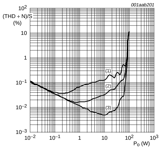
Fig 10. (THD + N)/S as a function of output power; SE configuration with 2 × 6 Ω load.
