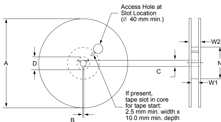
Figure 27. PowerSSO-16 reel 13"
