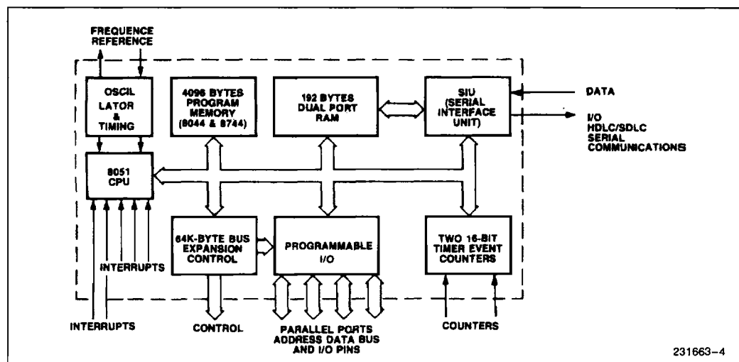
Figure 4. Block Diagram
