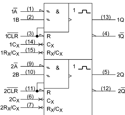
74VHC221AFT
