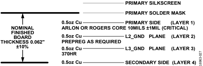
Figure 27. 4-Layer Stackup
