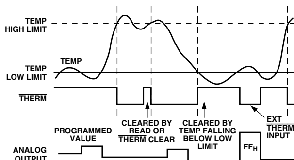
Figure 16a. \overline{\text{THERM}} Output in Default Mode
