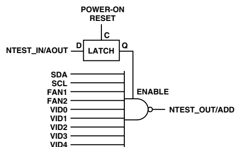
Figure 17. NAND Tree
