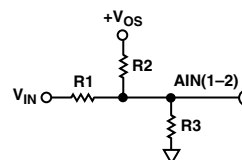
Figure 6. Scaling and Offsetting AIN(1-2) for Bipolar Inputs
