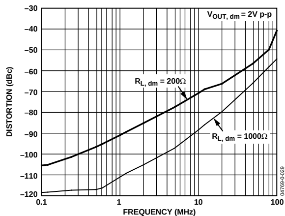
Figure 11. Second Harmonic Distortion at V_S = \pm 5\text{ V} at Various Loads
