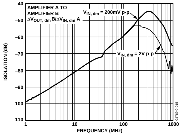
Figure 23. Amplifier-to-Amplifier Isolation vs. Frequency
