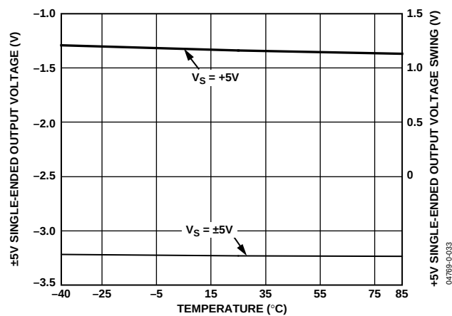
Figure 32. Negative Output Saturation Voltage vs. Temperature
