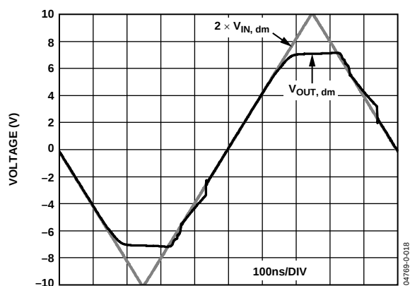
Figure 13. Overdrive Recovery
