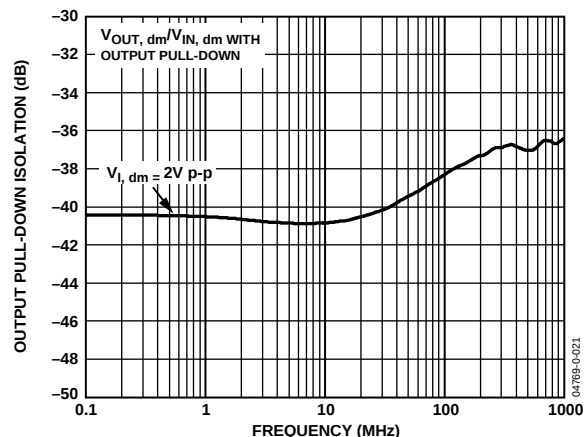
Figure 20. Output Pull-Down Isolation vs. Frequency
