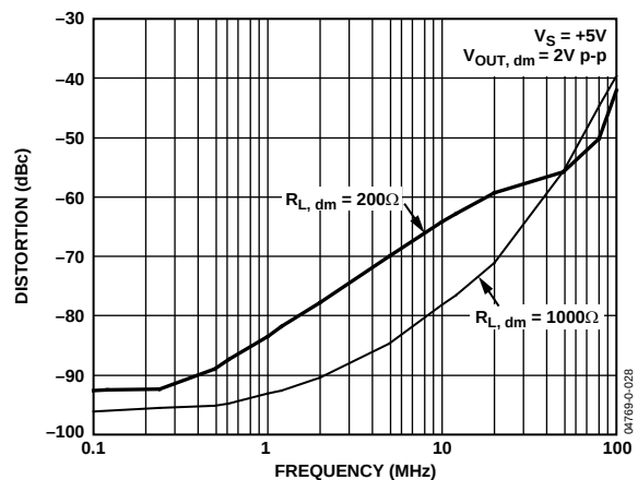
Figure 10. Third Harmonic Distortion at V_S = 5\text{ V} at Various Loads
