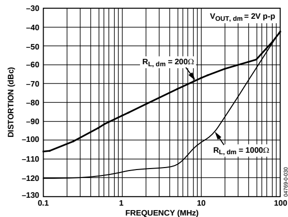
Figure 14. Third Harmonic Distortion at V_S = \pm 5\text{ V} at Various Loads
