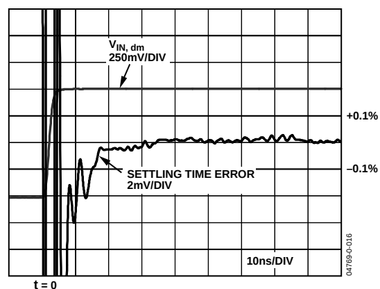
Figure 16. Settling Time (0.1%)
