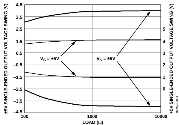
Figure 29. Output Saturation Voltage vs. Single-Ended Output Load
