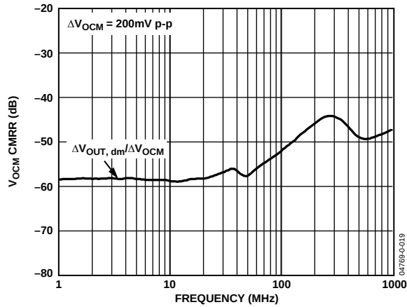
Figure 24 V_{OCM} CMRR vs. Frequency
