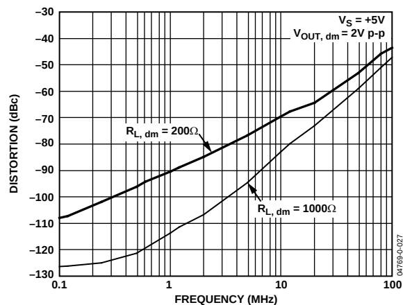
Figure 7. Second Harmonic Distortion at V_S = 5\text{ V} at Various Loads
