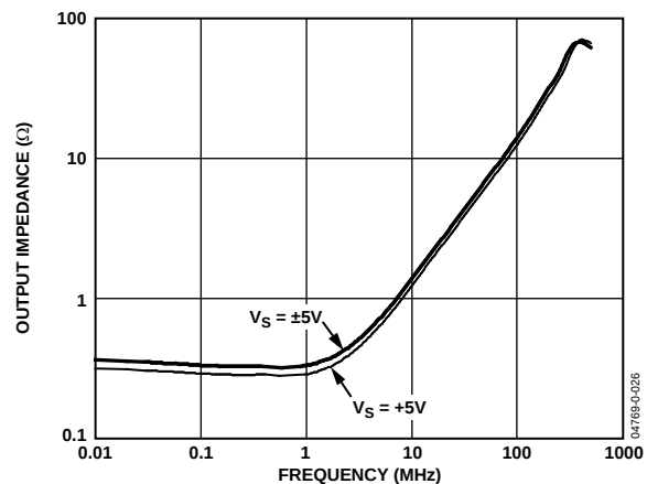
Figure 31. Single-Ended Output Impedance Magnitude vs. Frequency
