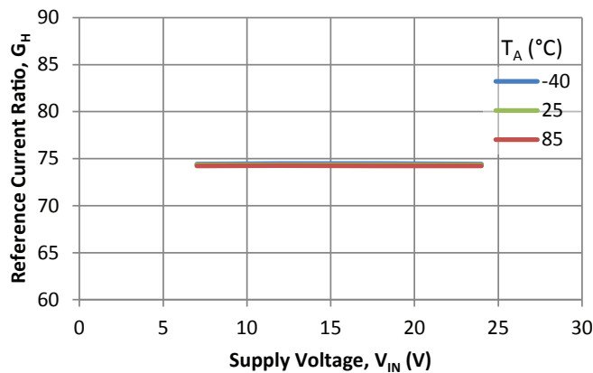
G_H vs. V_{IN} ( I_{REF} = 2 mA)
