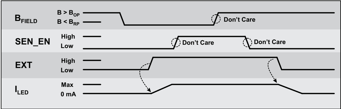
Figure 5: Overriding the Hall Sensor with EXT
