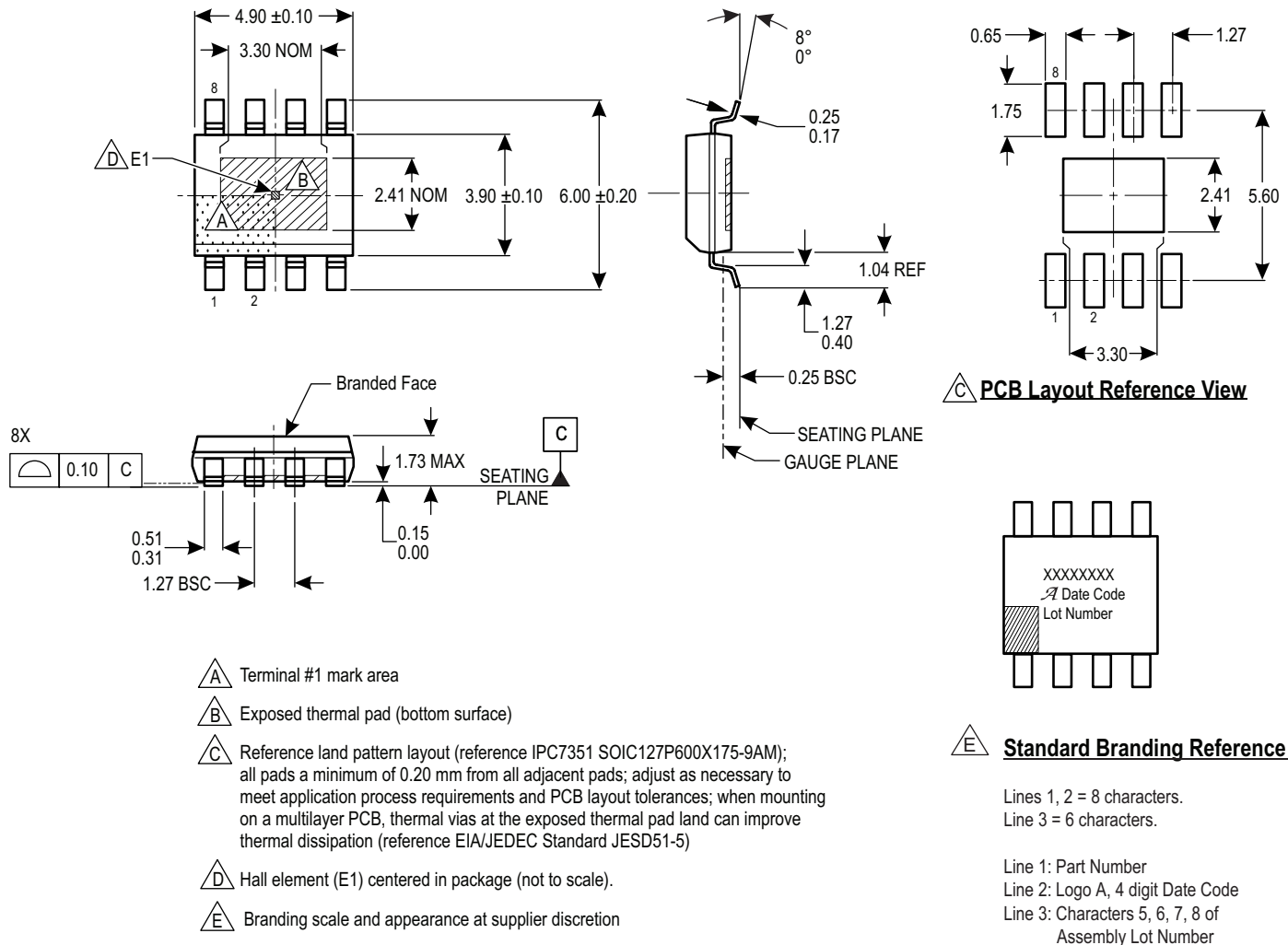
Figure 14: Package LJ, 8-Pin SOICN with Exposed Thermal Pad
