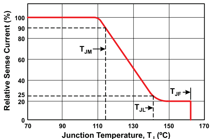
Figure 9: Temperature Monitor Current Reduction
