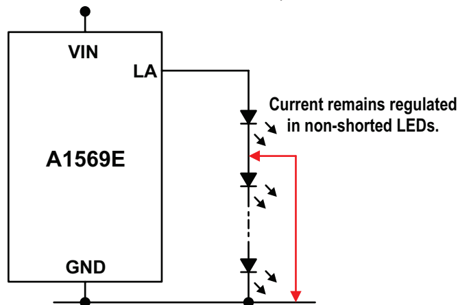
Figure 6: Any Cathode Short to Ground
