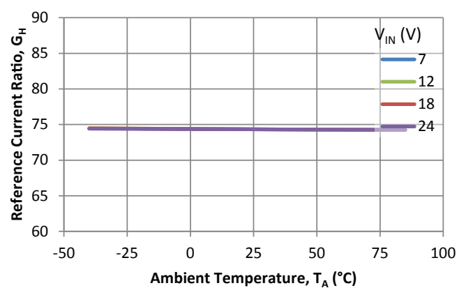
G_H vs. T_A ( I_{REF} = 2 mA)
