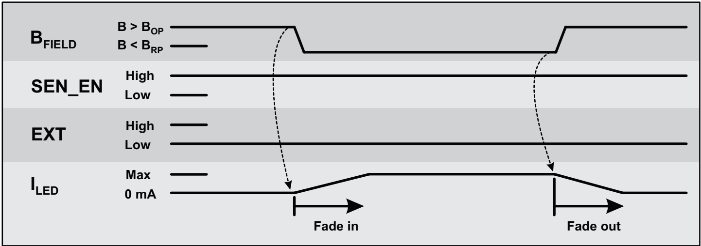
Figure 3: Hall-Activated Operation
