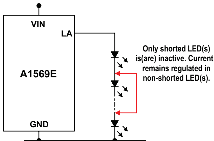
Figure 8: Shorted LED(s)
