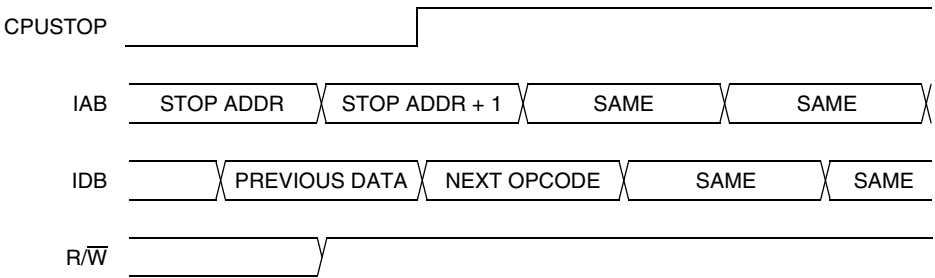
Figure 4-18. Stop Mode Entry Timing
