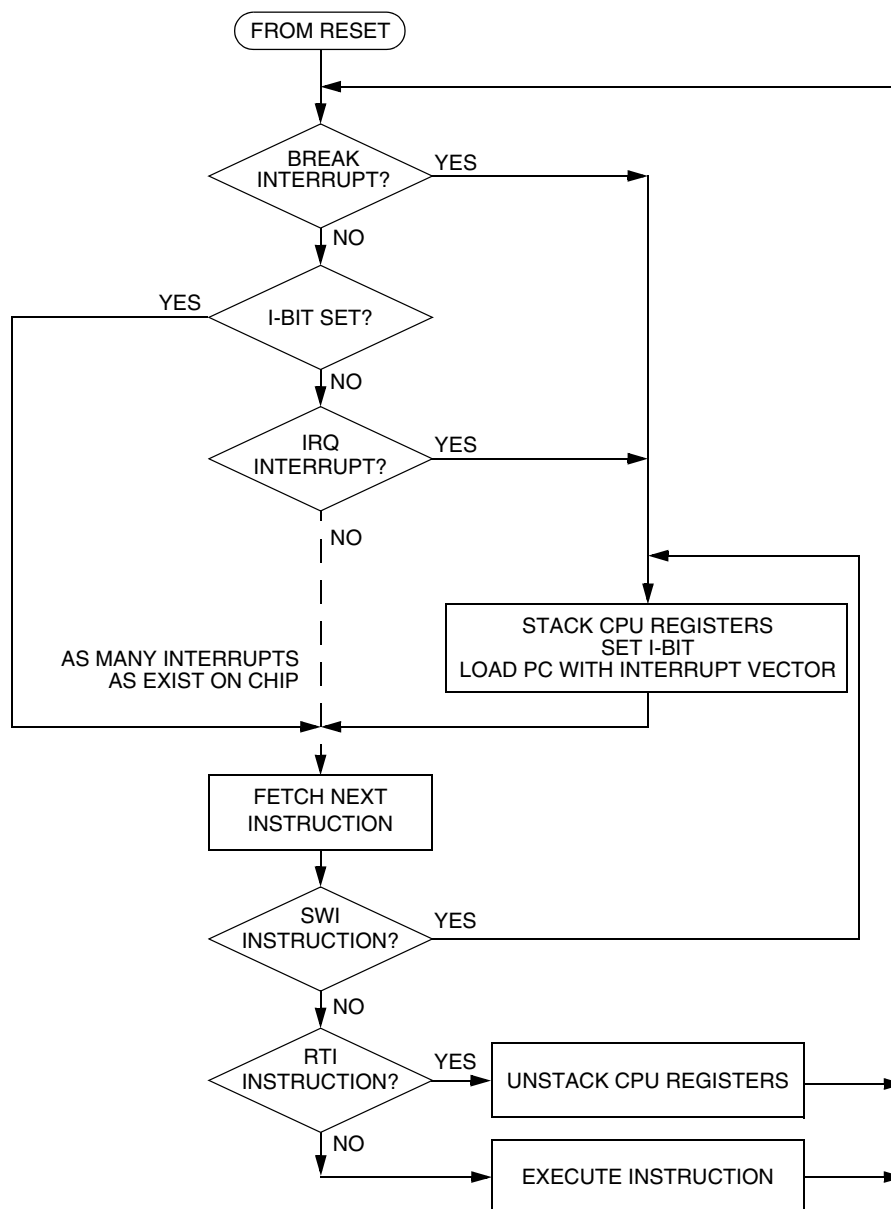
Figure 4-10. Interrupt Processing
