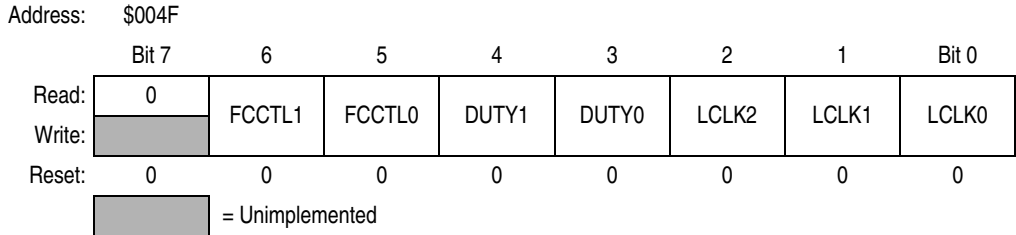
Figure 9-17. LCD Clock Register (LCDCLK)
